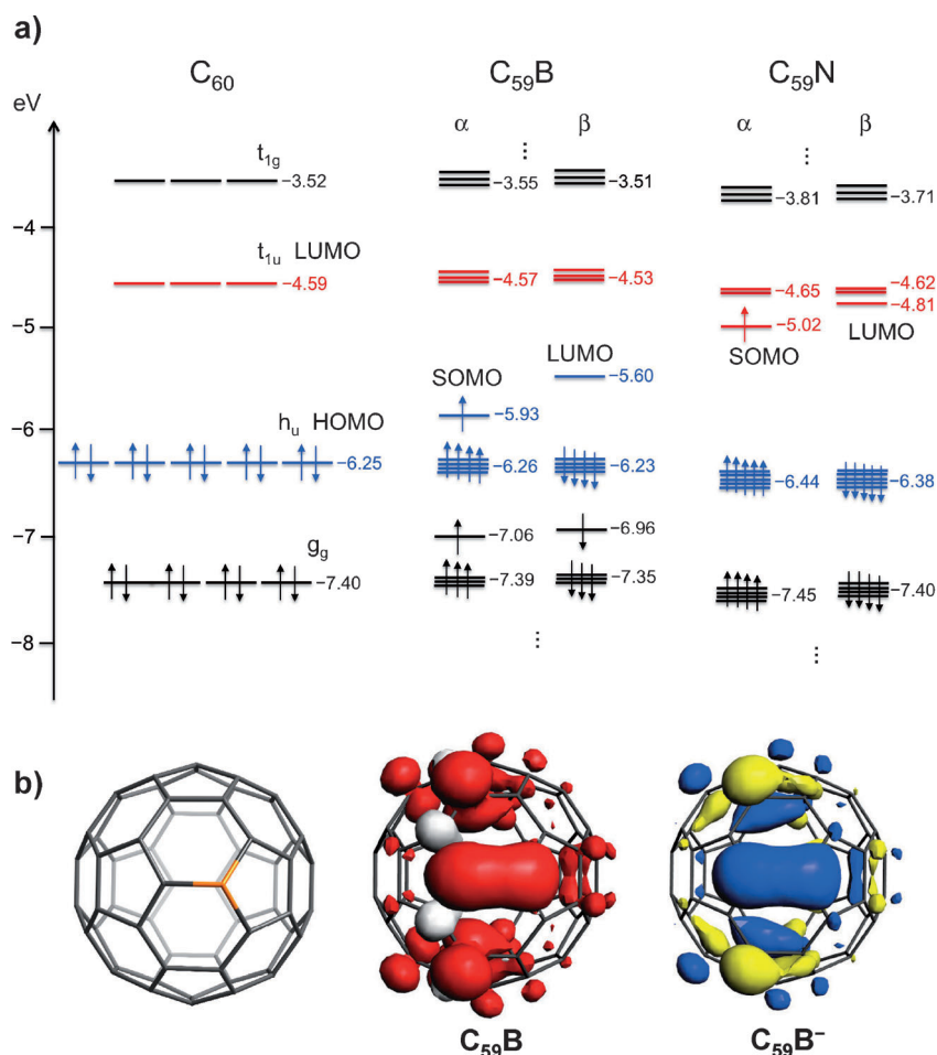
Figure 2. a) Molecular-orbital energy diagrams near the HOMO and LUMO of C_{59}B compared to I_h - C_{60} and C_{59}N . The HOMOs and LUMOs of I_h - C_{60} are broken into five (blue) and three (red) non-degenerate orbitals for C_s - C_{59}X ( X=B and N ) heterofullerenes. b) Representations of spin density for neutral C_{59}B (red and white), and the topology of the HOMO for C_{59}B^- (yellow and blue).
